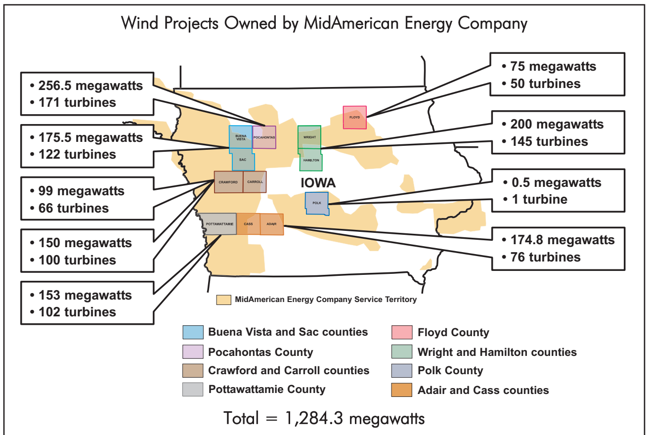
One of MidAmerican Energy Company's wind projects in Iowa
